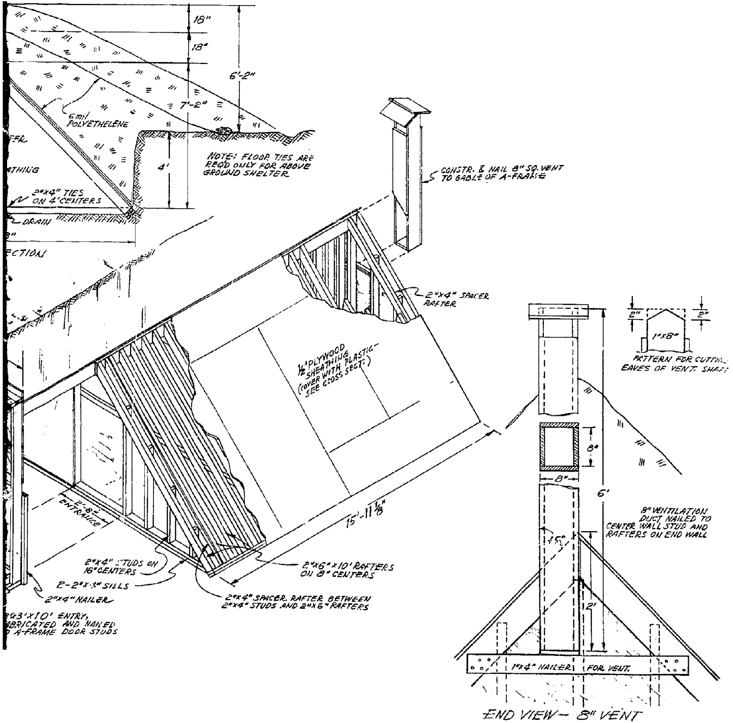
Fig. A-6.1. Two-Family, A-Frame Lumber Shelter
